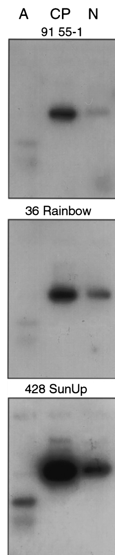
Figure 2. Comparative nuclear run-on transcription assays of nuclei isolated from leaves of CP hemizygous 55-1 and Rainbow and CP homozygous SunUp transgenic papaya. Nuclear transcripts of Rainbow 36 and SunUp 428 plants were hybridized with ^{32} P labeled probes specific to Actin (A), PRSV HA 5-1 coat protein (CP), or NPTII (N) genes. The CP/A ratio of labeled transcript for each run-on was 1.7, 2.0, and 3.8 for 55-1, Rainbow 36, and SunUp 428, respectively. Note that northern blots were also done for Rainbow 36 and SunUp 428 plants as shown in Figure 3.
